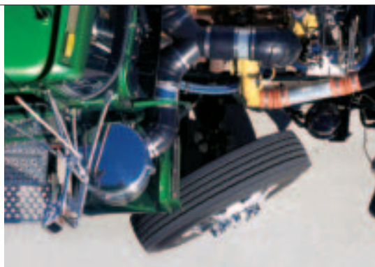
The T800's set-back front axle – together with steering geometry that delivers up to 54 degrees of wheel cut – helps drivers optimize and maneuver loads with ease.
