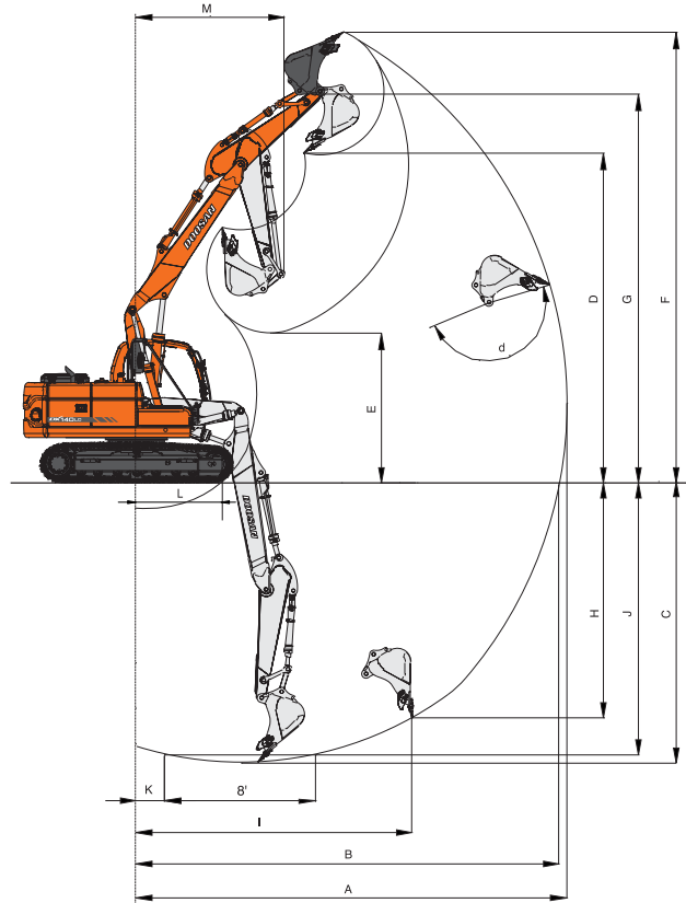
[ Two-piece Boom ]
