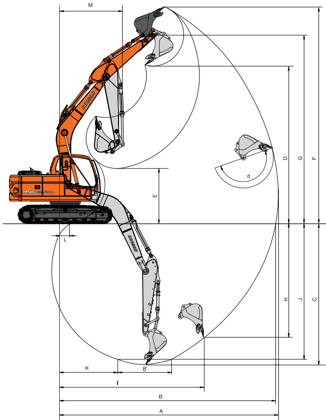
[ One-piece Boom ]
