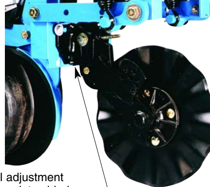
Unit mounted no-till couler cuts an opening directly in front of the double discs in tough soil conditions. Available in several blade choices to fit your soil conditions.
