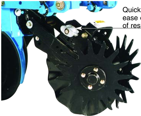
Unit mounted no-till couler/residue manager combo. To first move residue between rows then cut an opening for the row unit.
