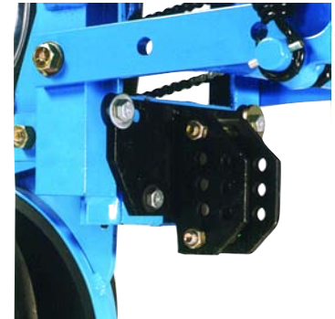
Monosem no-till row unit has standard face plate bolt-on mounting to accommodate any unit-mounted no-till or fertilizer attachment that is on the market today or will be in the future.
