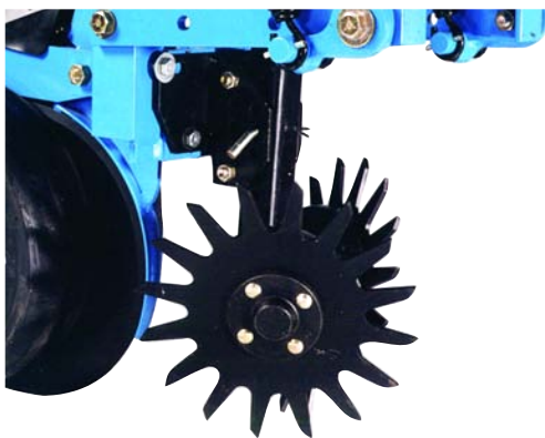
Unit mounted residue manager moves residue (not soil) to give planter gauge wheels a level surface.
